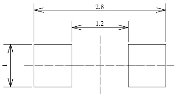
Symmetrical pad
