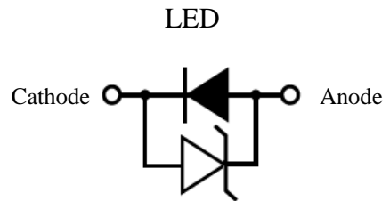
Protection diode
