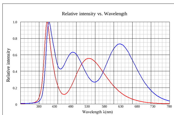
Fig.5 Spectral differences in white LEDs
