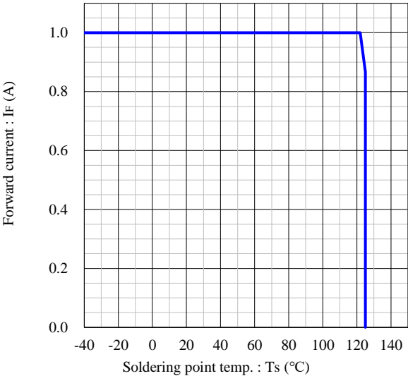
Maximum ratings of forward current
