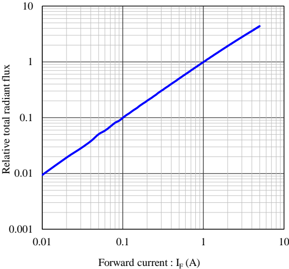
Forward current vs. Relative total radiant flux
