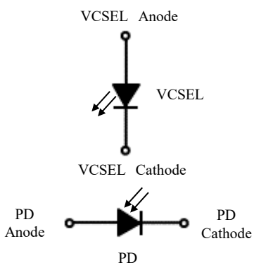
Inside circuit
