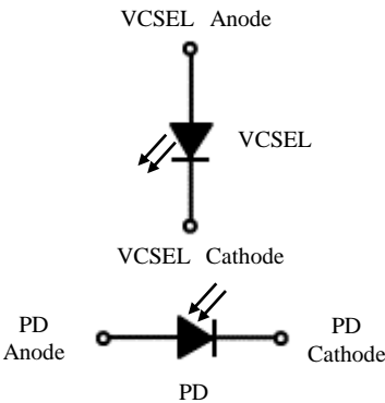
Inside circuit
